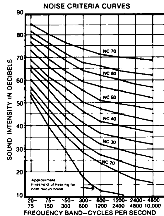
Each NC curve connects points of equal acceptability
